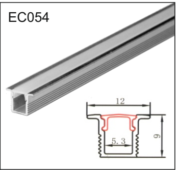
5mm CONCEALED
