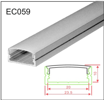
25mm SURFACE
